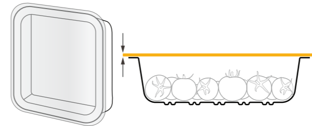
Outside cut: The top film is cut along the inside of the tray rim dimensions.
