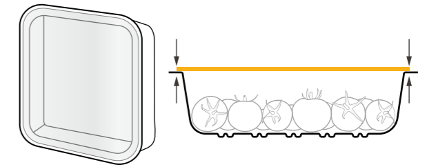
Inside cut: The top film is cut along the inside of the tray rim dimensions.
